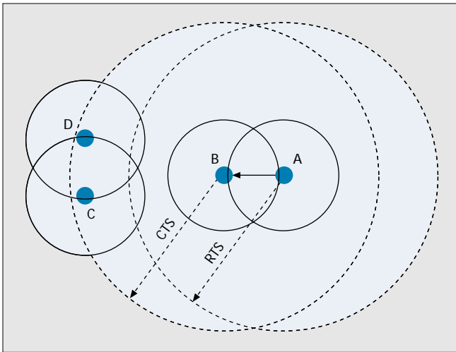
Figure 1. Inefficiency of the standard RTS-CTS approach. Nodes A and B are allowed to communicate, but nodes C and D are not. Dashed circles indicate the maximum transmission ranges for nodes A and B, while solid circles indicate the minimum transmission ranges needed for coherent reception at the respective receivers.
