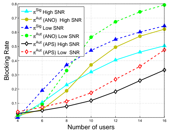
Fig. 10: User blocking rate of the \pi^{Aut} and \pi^{Sig} methods as a function of Number of users I .
