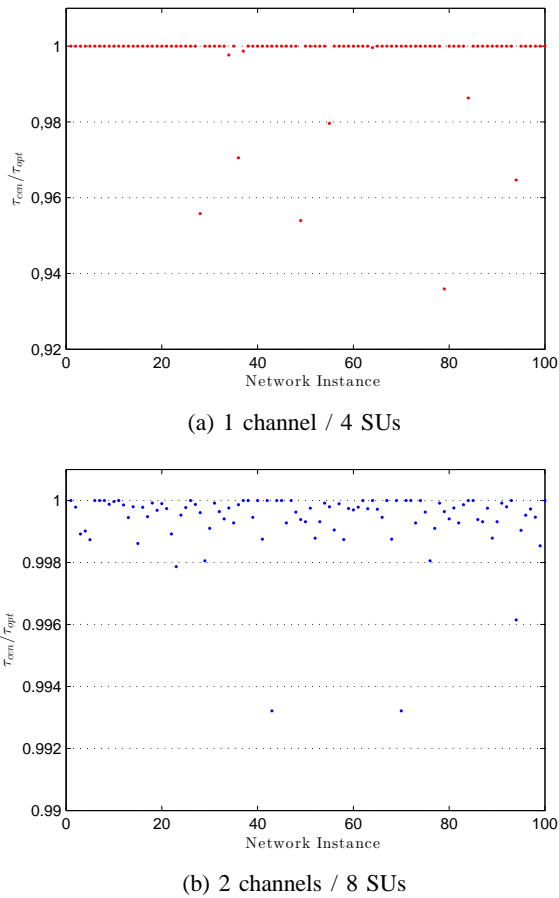
Fig. 3: Ratio of time average data rate of the \pi^{Cen} subchannel assignment to the optimal assignment.
