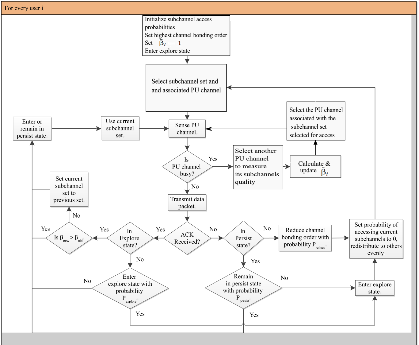
Fig. 2: \pi^{Aut} Method.
