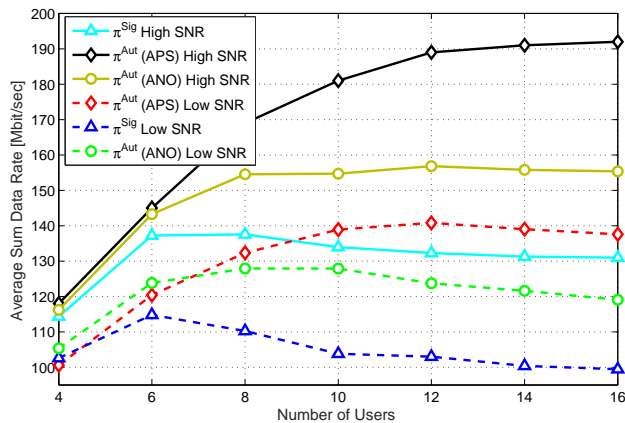
Fig. 5: Average sum data rate achieved by the \pi^{Aut} and \pi^{Sig} methods vs. number of users, with |\mathcal{S}_p| = 8 , N_R = 50 meters, and users with heterogeneous CB capabilities, i.e., maximum CB capabilities are uniformly selected from O_{max,i} = 1 to O_{max,i} = |\mathcal{S}_p| .
