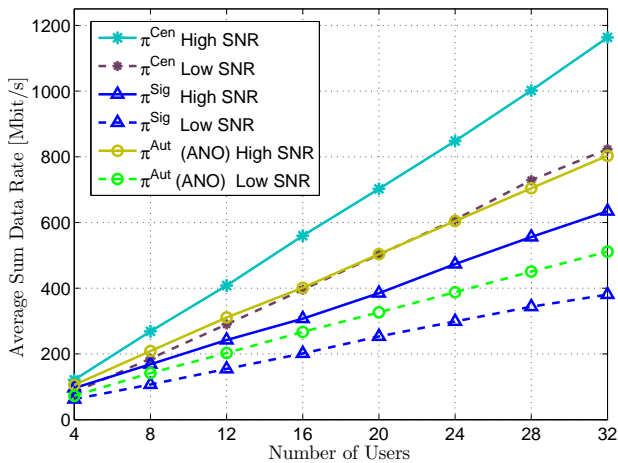
Fig. 9: Average sum data rate vs. number of users I for the \pi^{Aut} , \pi^{Sig} and the \pi^{Cen} methods. Number of subchannels is increased with the number of users, i.e., |S_p| = I .
