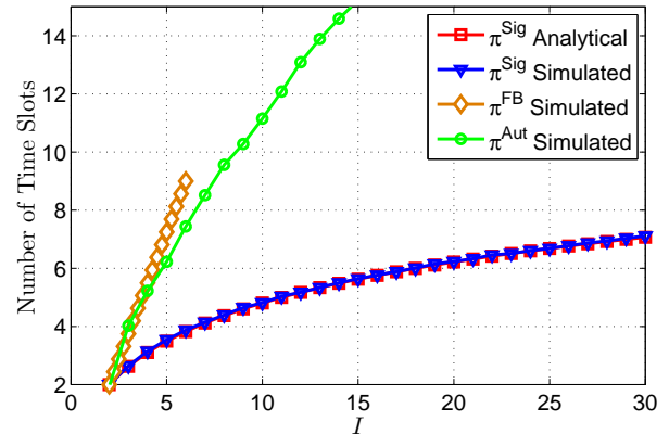
Fig. 4: Expected time to converge to conflict free subchannel selections of the \pi^{Sig} and \pi^{FB} methods as a function of I users, under collision-protocol model. The number of available subchannels |\mathcal{S}_p| = I , and O_{max,i} = 1 \forall i .
